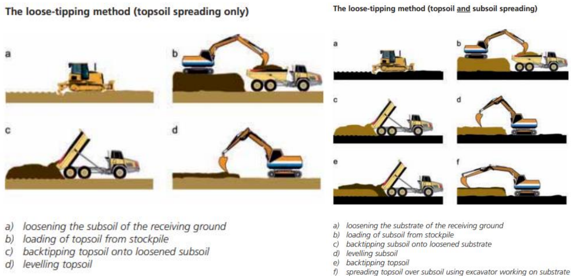
Figure 5-4. The loose-tipping method of soil reinstatement
